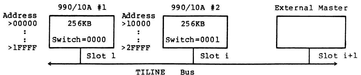
Figure A-2. Improperly Configured Multiprocessor Memory
